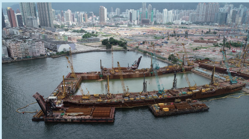
九龍灣的第一階段臨時圍堰 Stage 1 temporary cofferdam at Kowloon Bay
